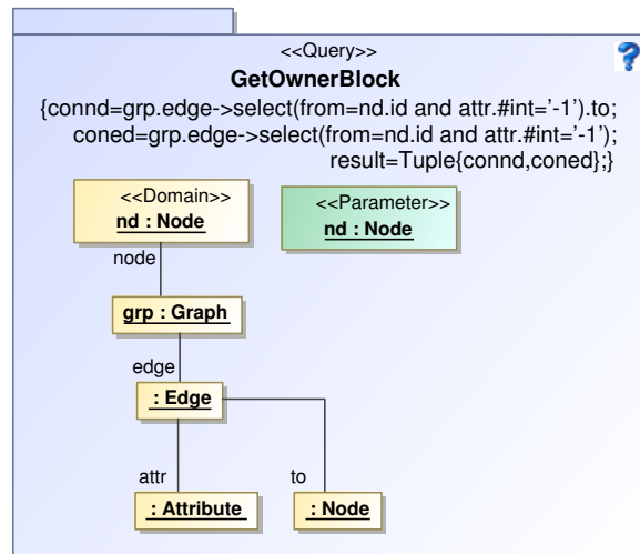
Figure 20: Get owner block of a node
