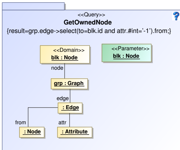
Figure 19: Get owned nodes of a block
