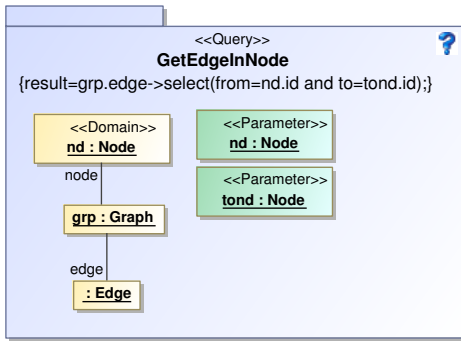
Figure 15: Get edges between nodes
