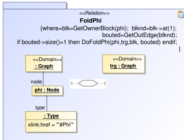
Figure 7: Select a Phi owned by a block with only out control edge (relName: FoldNode )
